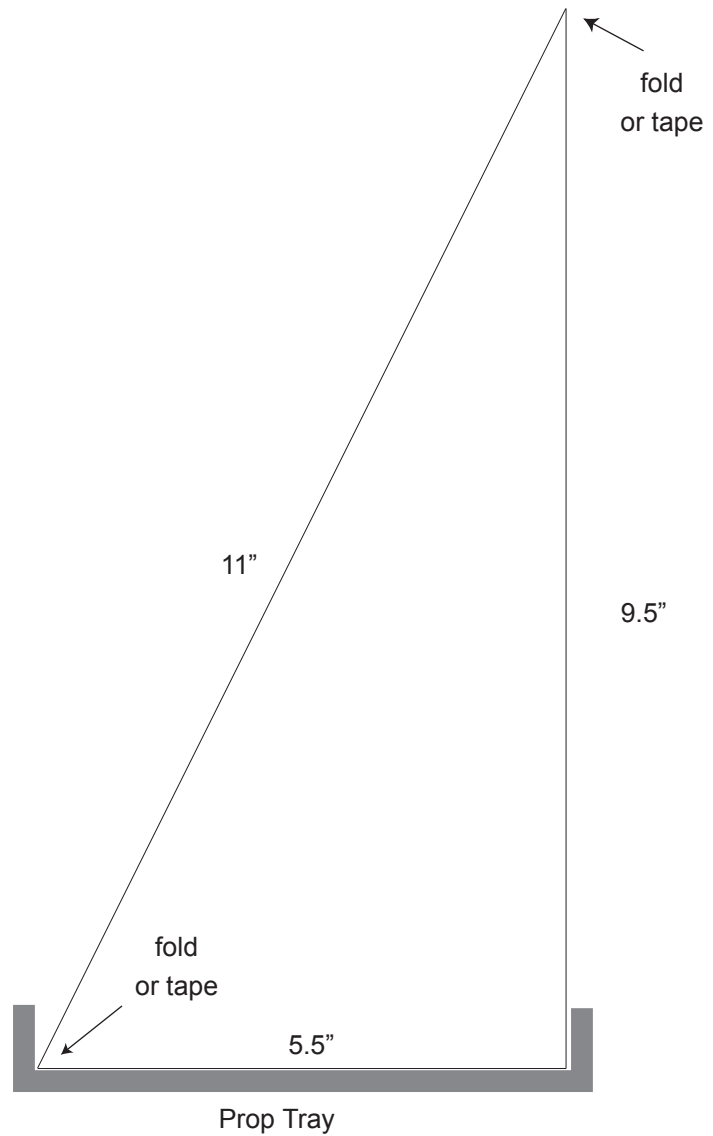
Cross section showing script holder in prop tray.
